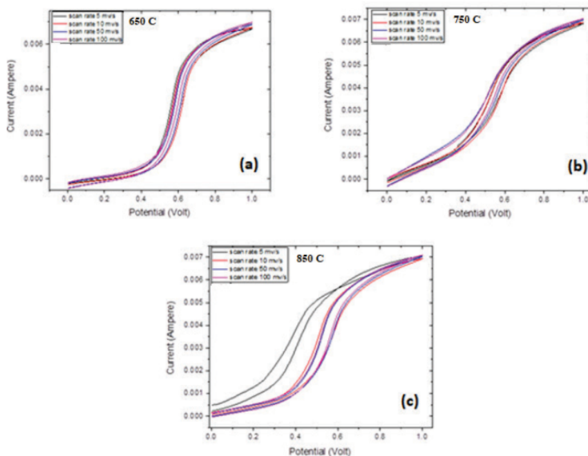
Fig. 4. CV curve of Borassus Flabelifer L at (a) 650°C, (b) 750°C, and (c) 850°C.
