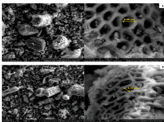
Fig. 3. SEM Image of Borassus Flabelifier L by heating at (a) 650 o C and (b) 750 o C.
