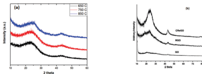
Fig. 2. XRD Data of (a) Borassus Flabelifier L at Various Temperature of Heating (b) RGO phase determined from natural Graphite (Sungjin Park, et al, 2011).
