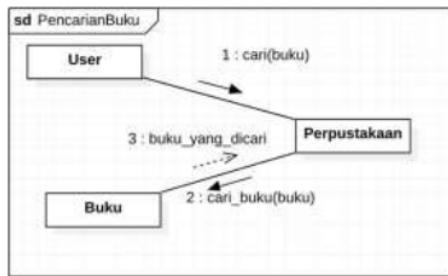
Gambar 1 Contoh Communication Diagram 1 (CD1)
