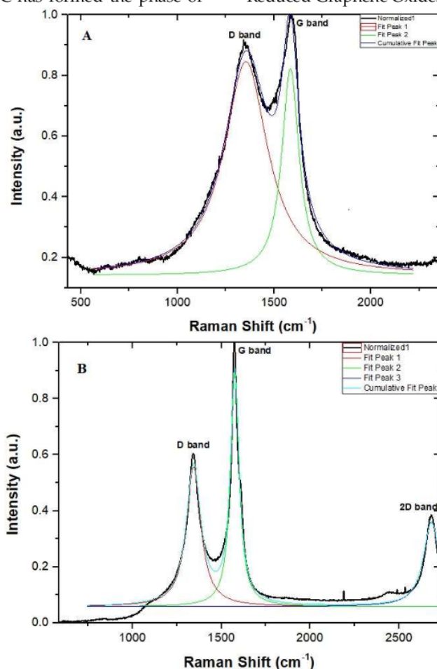
Figure 4 Raman Spectroscopy Curve Fitting of activated Borassus Flabelifer at (a) 650 °C and (b) 950 °C
