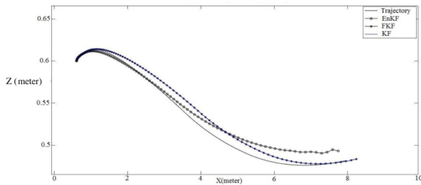
Figure 7. The estimation of trajectory 2
