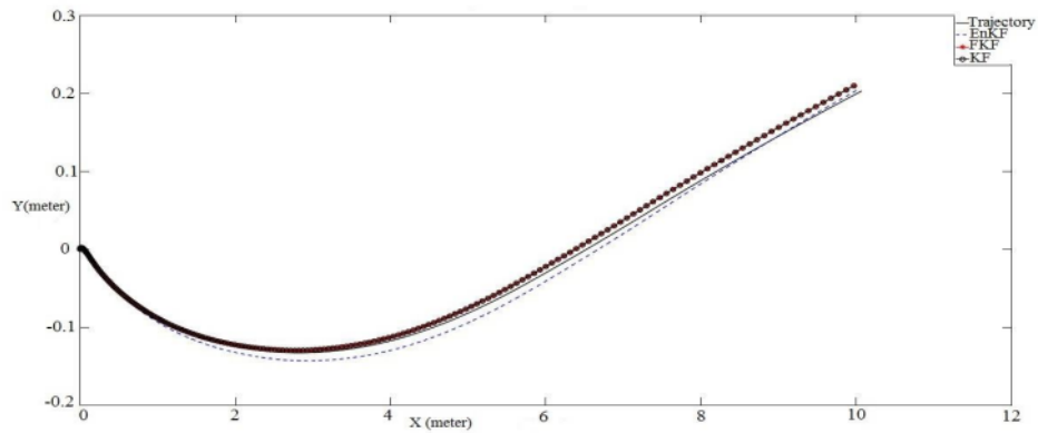
Figure 6. Estimation of trajectory 1.
