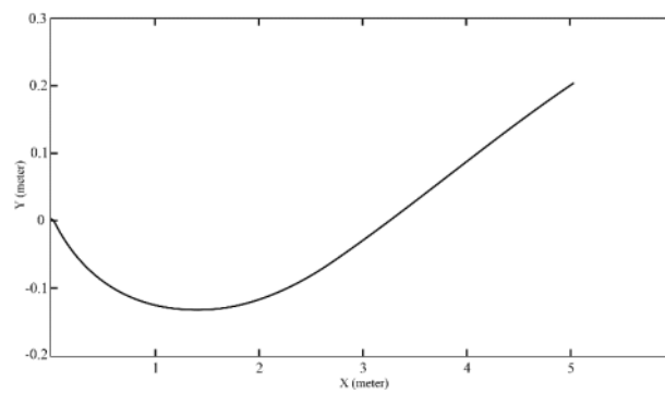
Figure 3. Turning trajectory.
