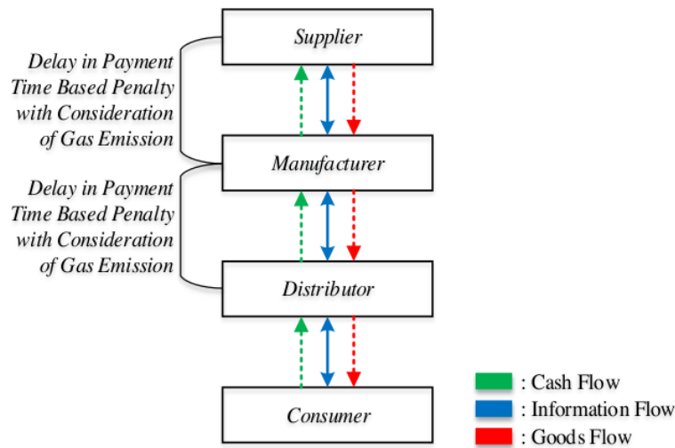
Fig. 1. Conceptual Model
