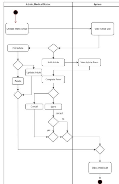
Figure 6. Activity diagrams of the admin and doctor process managing article data
