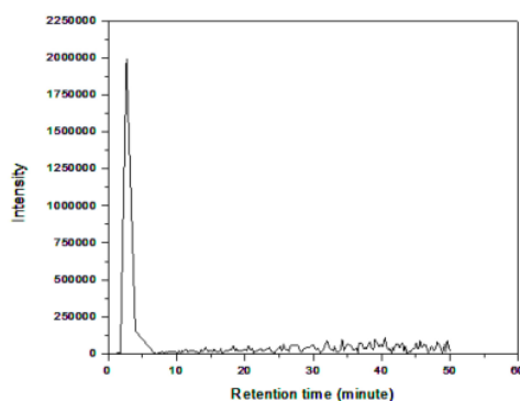
Fig. 2. High Pressure Liquid Chromatography of Bassella rubra linn leaf extract
