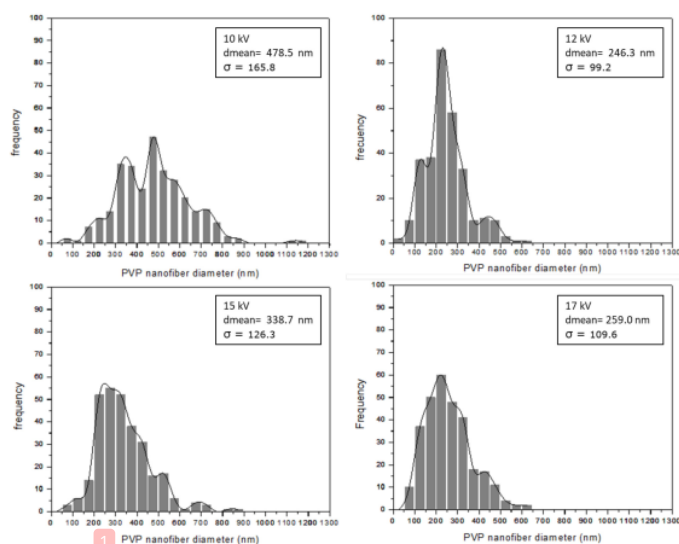
Fig. 4. PVP nanofiber diameter size distribution
