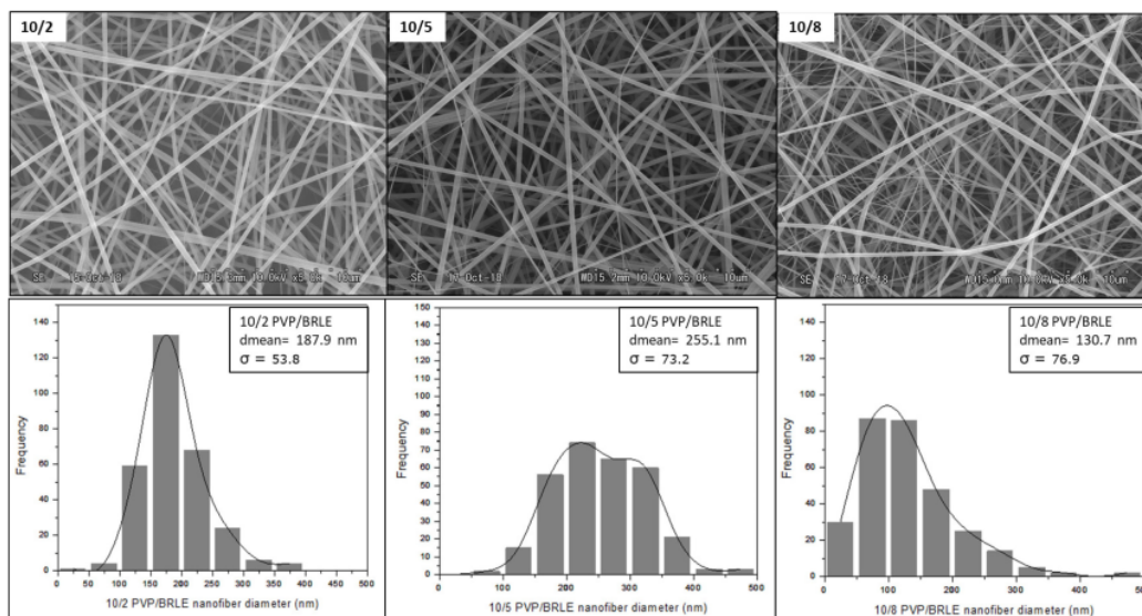
Fig. 5. SEM image and nanofiber diameter of PVP/BRLE at various composition
