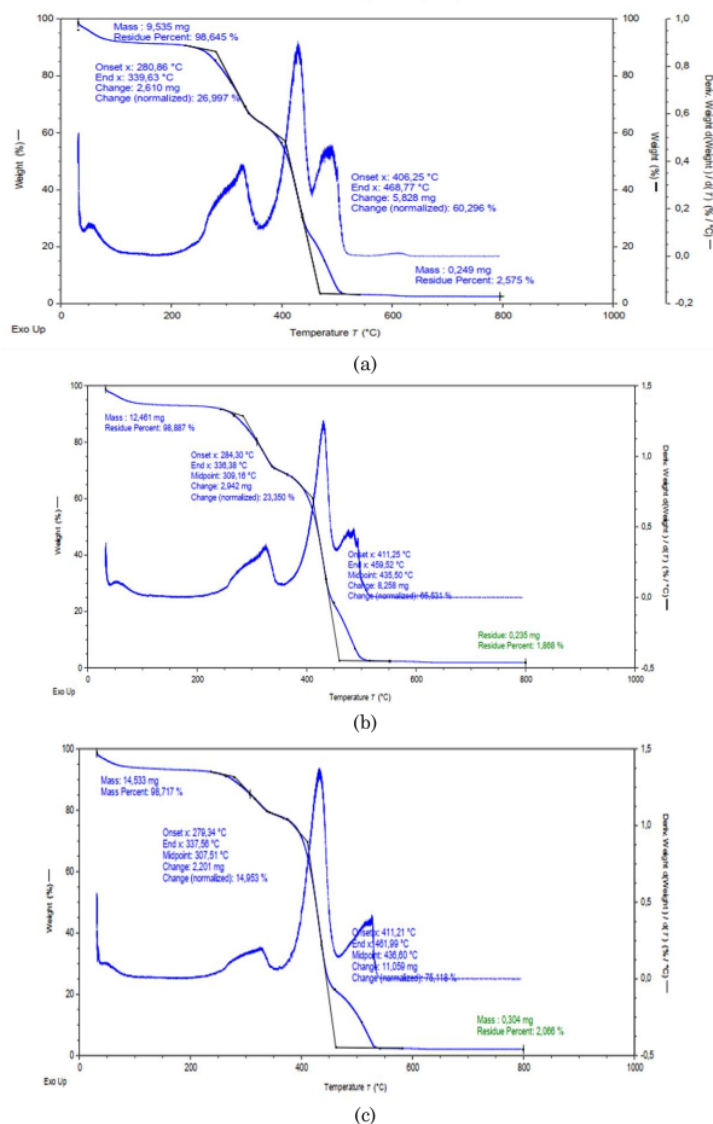
Fig. 5 TGA Result for RDF Pellet Samples from Garden and PET Waste with composition PP-25% (a), PP-50% (b), and PP-75% (c)
