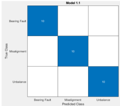
Fig. 5. Linear SVM Confusion Matrix
