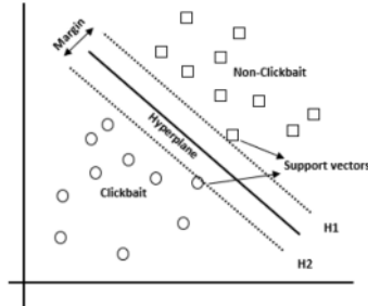
Fig. 1. Support Vector Machine [11]
