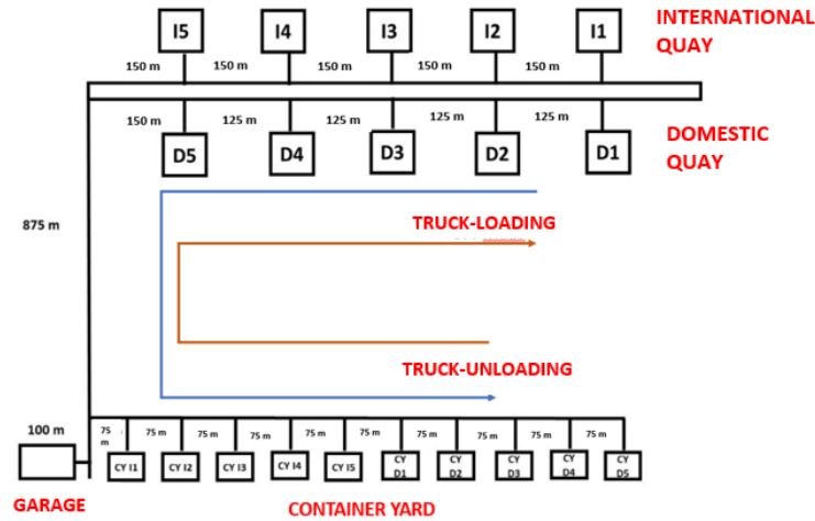
FIGURE 2. Container Terminal Layout
