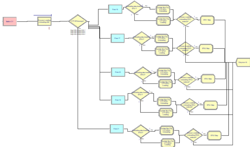
FIGURE 5. CY Sub-Model
