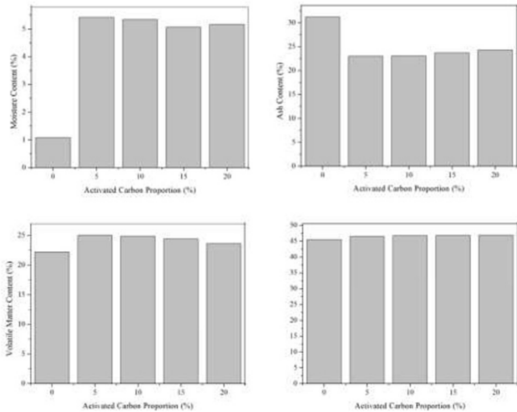
Fig. 5. Proximate analysis results.
